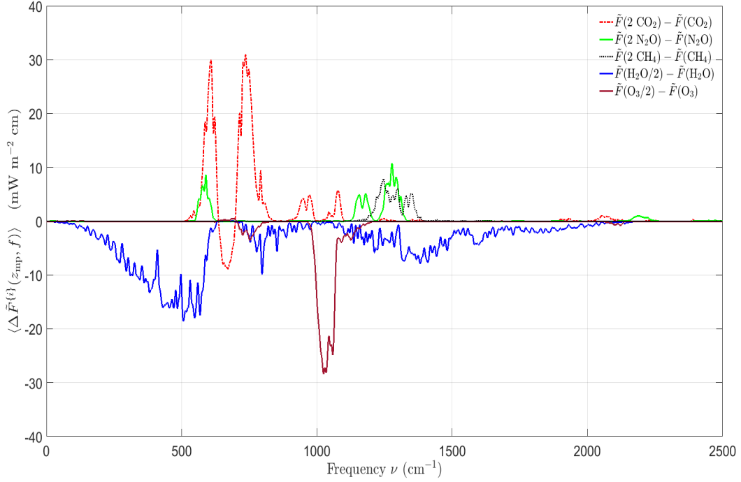
Figure 6: Spectral forcing increments (45) for doubled concentrations of \text{CO}_2 , \text{N}_2\text{O} and \text{CH}_4 . These are the magnified differences between the black and red curves of Figs. 4 and 5. For most frequencies \langle \Delta \tilde{F}^{\{i\}}(z_{\text{mp}}, 2) \rangle is positive. This is because doubling the concentrations of greenhouse gases shifts the emission heights z_e of (38) to higher, colder altitudes in the troposphere. An exception is the band of frequencies near the center of the exceptionally strong bending-mode band of \text{CO}_2 at 667 \text{ cm}^{-1} . Here doubling \text{CO}_2 moves the emission heights to higher, warmer altitudes of the stratosphere, where molecules can more efficiently radiate heat to space. Also shown are forcing increments for halved concentrations of \text{H}_2\text{O} and \text{O}_3 . Halving ensures that the relative humidity does not exceed 100%, and reduces the clutter of the graph.
