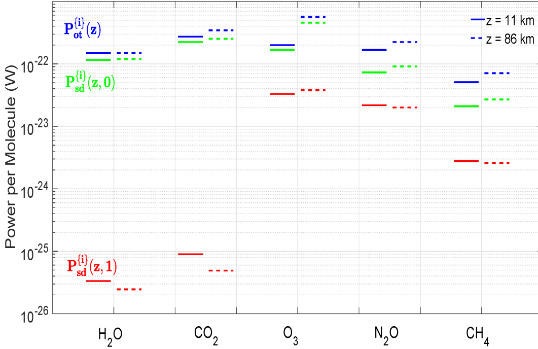
Figure 10: A graphical display of the per-molecule forcing powers of Table 4. At standard column densities the (red) powers, P_{sd}^{\{i\}}(z, 1) , for H_2O and CO_2 are suppressed by four orders of magnitude from their values in the optically thin limit (blue) where the powers are P_{ot}^{\{i\}}(z) . This is due to strong saturation of the absorption bands. Saturation effects (difference between the blue and red lines) are much less for the minor gases, O_3 , N_2O and CH_4 . The green lines are the powers per molecule, P_{sd}^{\{i\}}(z, 0) , of the i th greenhouse gas in its low-concentration limit, but when the forcing power is suppressed by other gases at their standard densities. Interference effects (difference between the blue and green lines) are more pronounced for N_2O and CH_4 than for H_2O and CO_2 . Fig. 2 shows the strongest bands of O_3 overlap little with those of other greenhouse molecules, minimizing interference effects.
