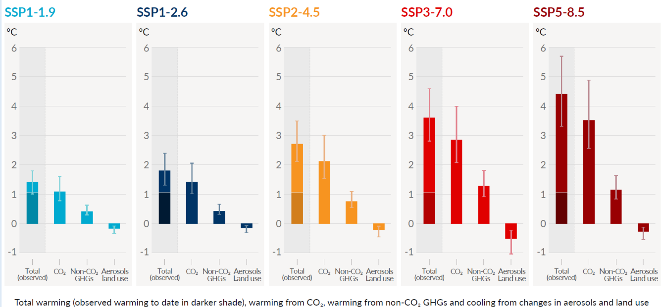
Figure 1: Five scenarios from the Summary for Policy Makers in the Sixth Assessment Report (AR6) in 2021.
