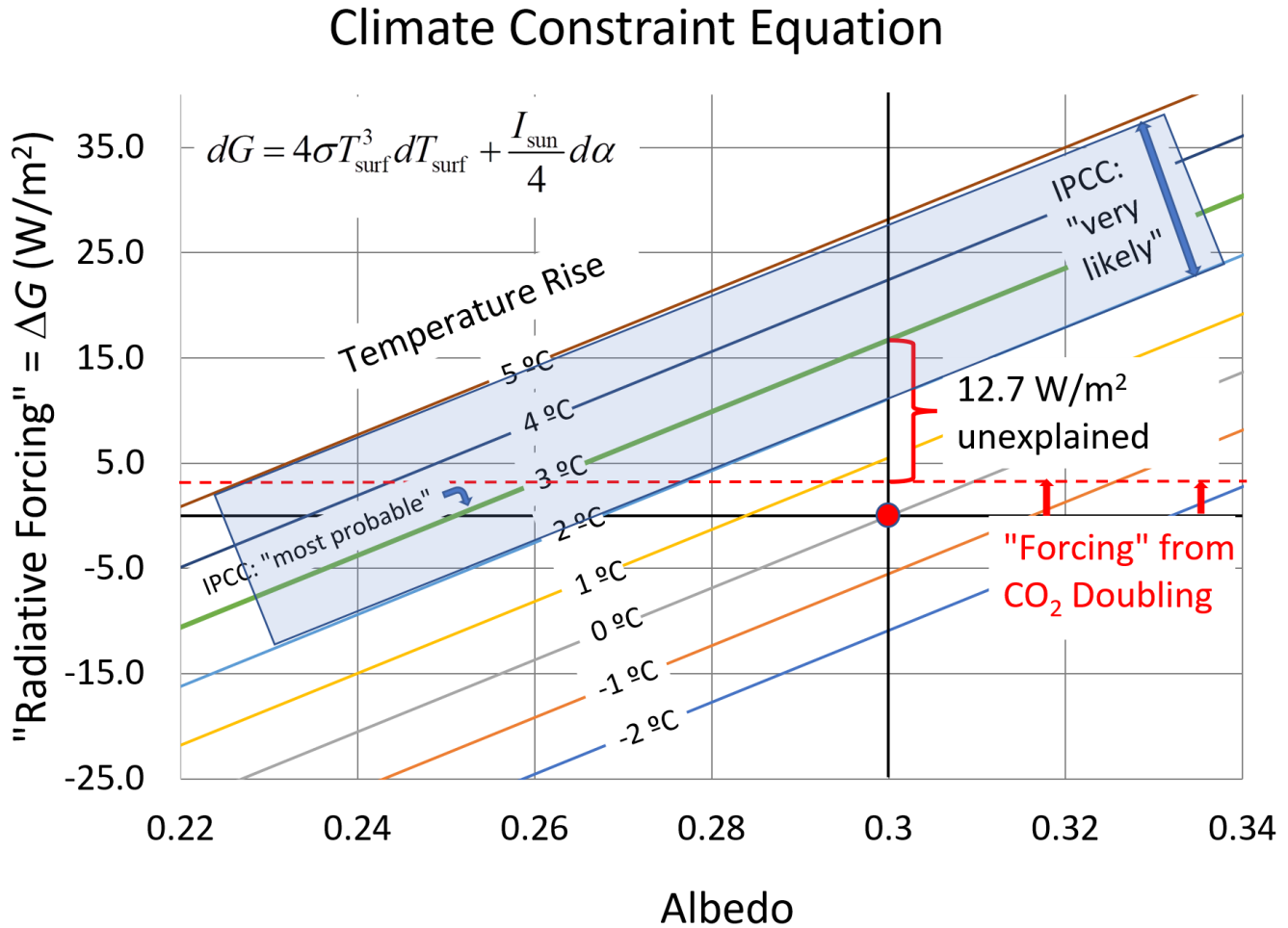
Figure 1: The differential form of the climate constraint equation. The red dot shows the current situation. The dashed red line shows the “radiative forcing” ( =3.47 \text{ W/m}^2 , IPCC) due to doubling \text{CO}_2 concentration, and the green slanted line shows IPCC’s “most probable” temperature rise of 3^\circ\text{C} . IPCC says that the rise due to doubling is “very likely” to be between 2^\circ\text{C} and 5^\circ\text{C} . A temperature rise dT_{\text{surf}} of 3^\circ\text{C} will increase surface radiation by 16.5 \text{ W/m}^2 . IPCC has no explanation and no description of how 3.47 \text{ W/m}^2 can cause 16.5 \text{ W/m}^2 of increased surface radiation.
