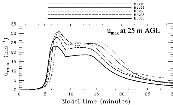
FIG. 5. A time series of maximum values of the u component of the horizontal wind at 25 m AGL for Mov00, Mov03, Mov06, Mov09, and Mov12.
