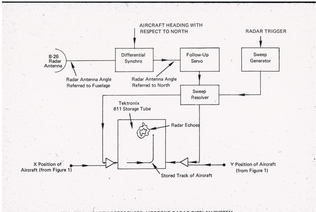
FIGURE 2 - EARTH REFERENCED AIRBORNE RADAR DISPLAY SYSTEM
