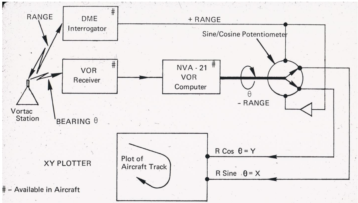
FIGURE 1 - TECHNIQUE FOR OBTAINING PLOT OF AIRCRAFT TRACK IN AIRCRAFT
